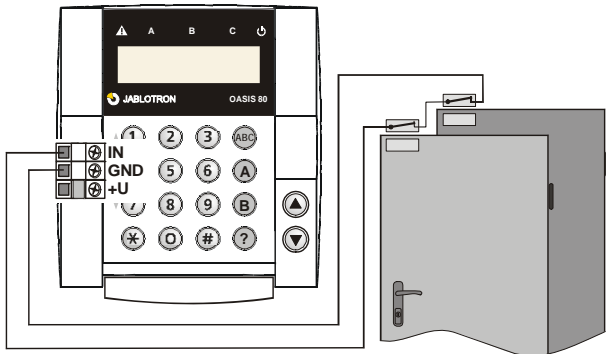
An example of door detector wiring.
